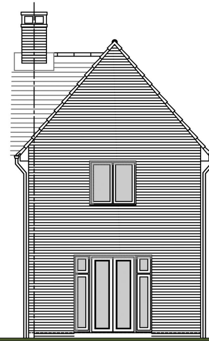
Rear Elevation
